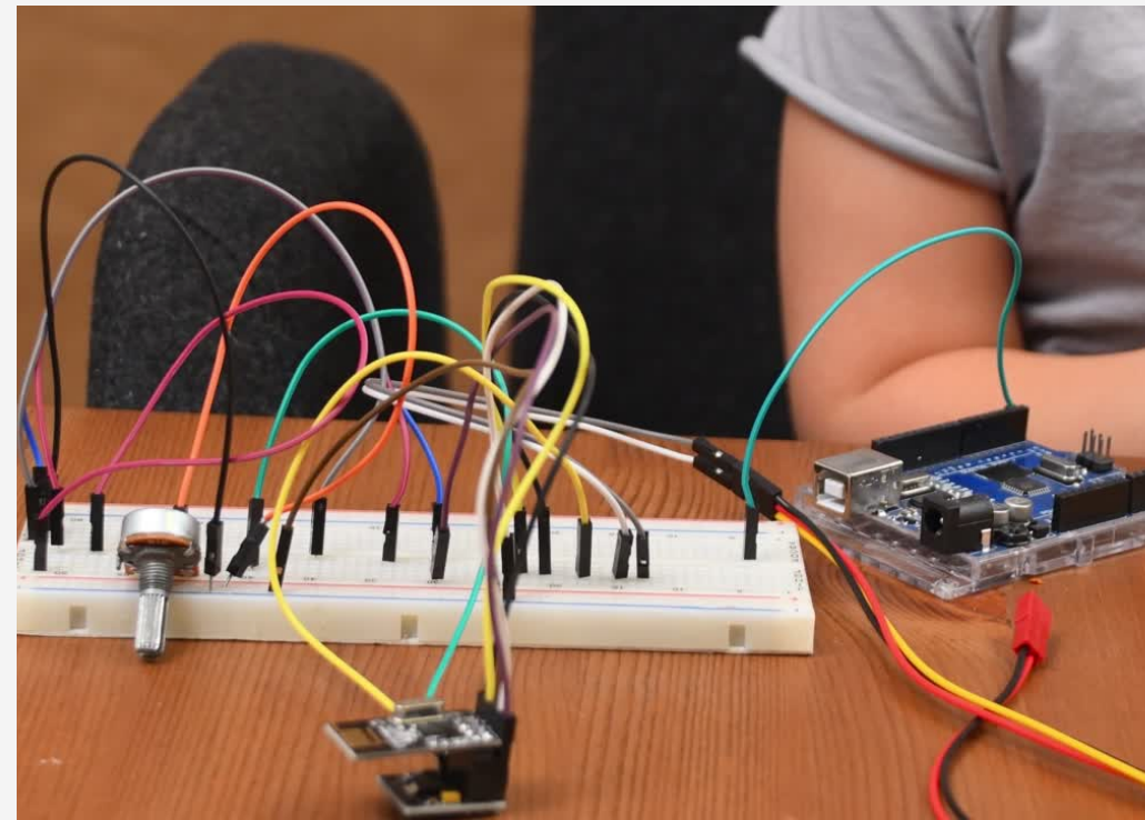
Breadboard
